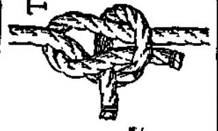
Sheet Bend with Seizing
